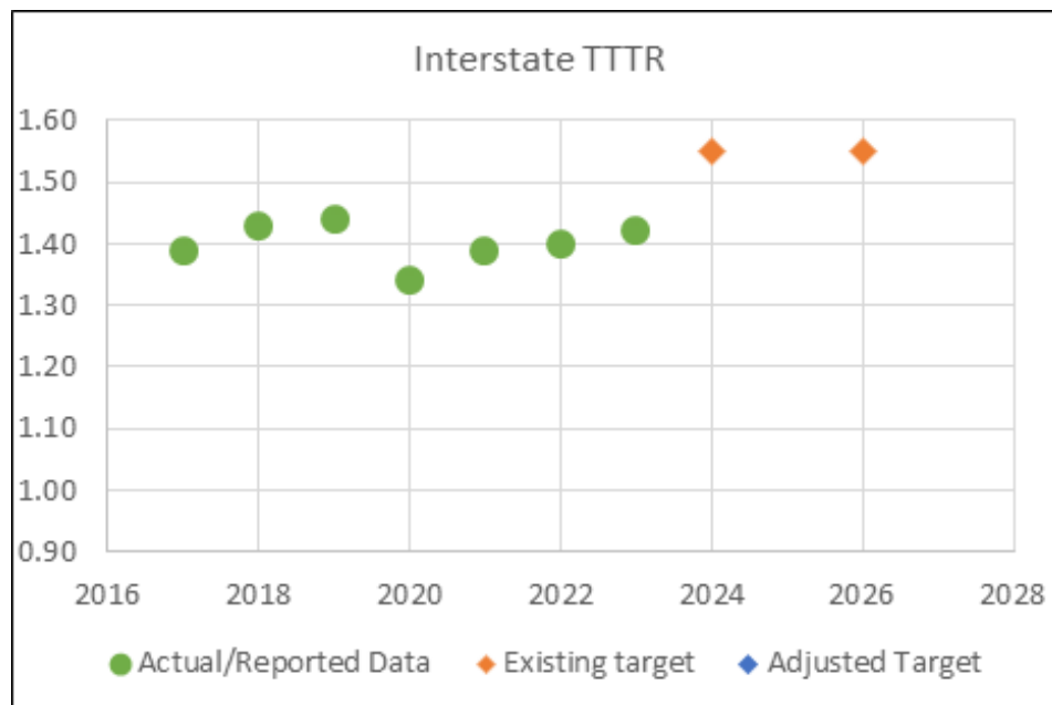
FIGURE 14: TRUCK TRAVEL TIME RELIABILITY IN TEXAS
